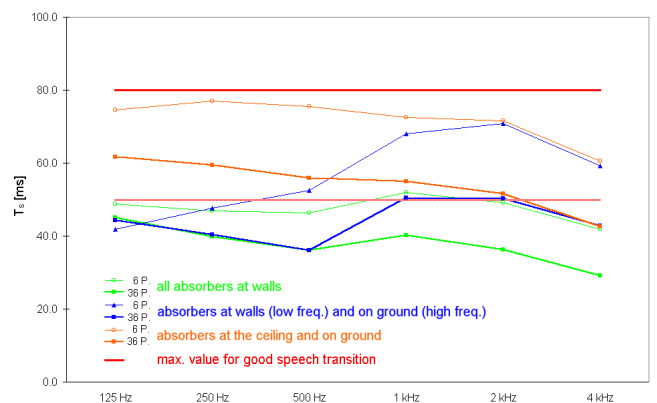
Figure 3: Effects of absorber position are studied by simulation of a conference room (10m x 14m x 3m) occupied by 6 or 36 persons. 3 versions, corresponding to a), b) and c) of fig.2, are compared, all with equal equivalent absorber surface. Results indicate that absorbers are most effective to reduce reverb times (mid graph) and center times (lower graph), when positioned at the walls.
