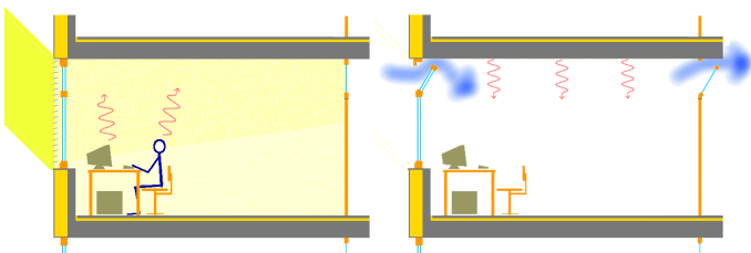
Figure 1: The basic concept of passive cooling - an office room shown as an example. During day (left) the room is heated by several sources: the sun, electric light, computers and other equipment, and the occupants. Part of this heat is stored into the massive concrete ceiling. During night (right) the room is vented by cool night air and the heat is unloaded from the ceiling. For good cooling effect the storage element (the ceiling) must show a large surface to the room at good thermal conductivity and high storage capacity. This prohibits acoustic absorbers covering the ceiling.
